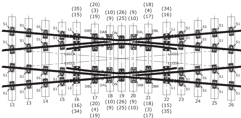
1:6 Diamond Crossing
