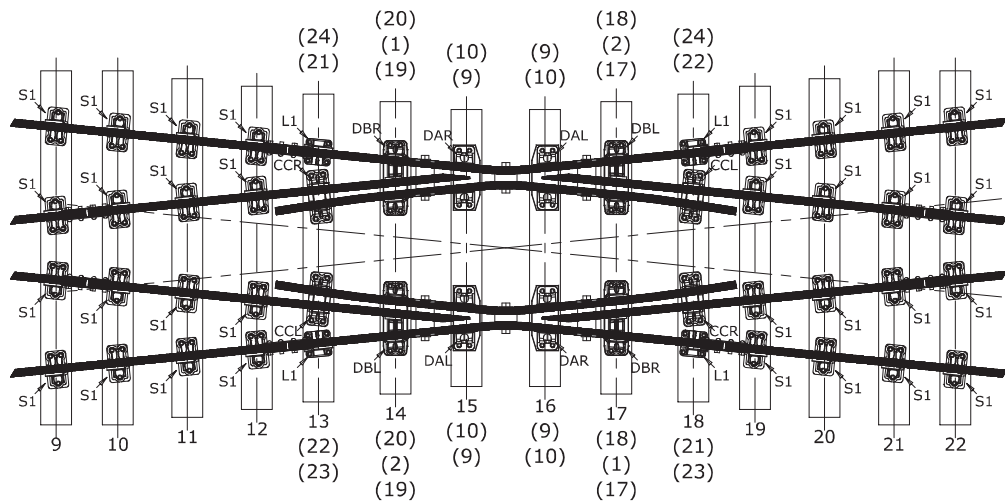
1:5 Diamond Crossing
